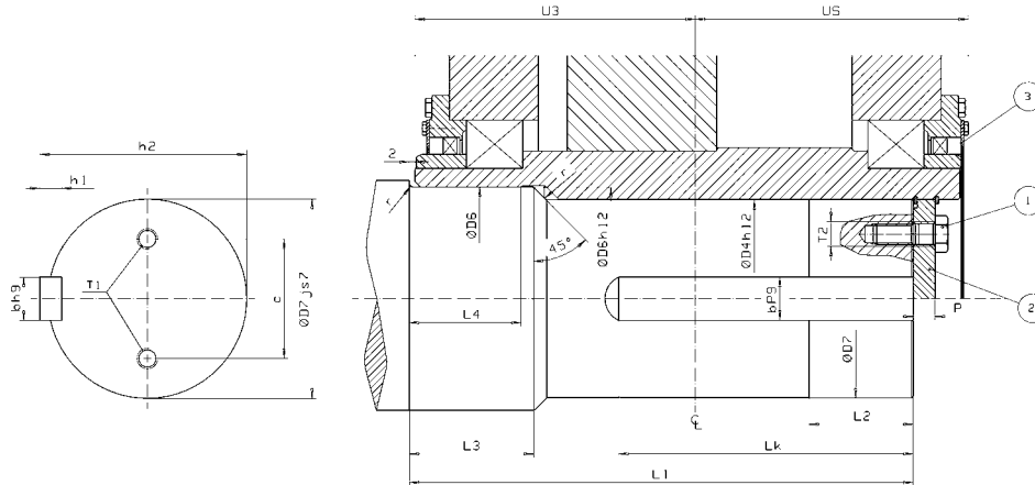
Shaft end
