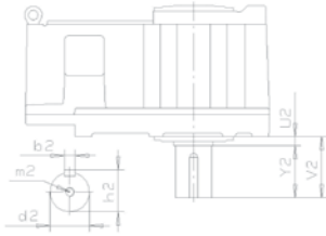
Type D4PVSF
